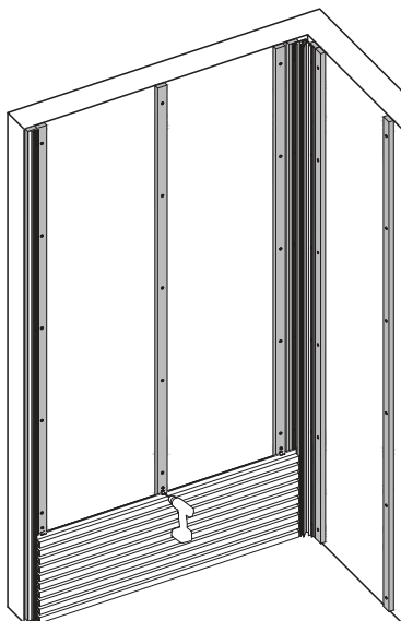
Horizontal boards on vertical battens
