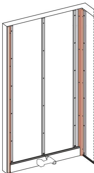
Horizontal boards on vertical battens
