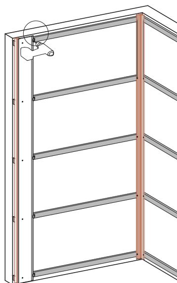
Vertical boards on horizontal battens
